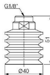
[ With 18FB fitting ]
