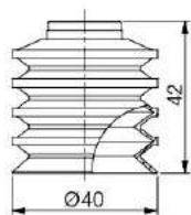
[ Rubber part ]
