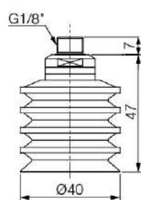
[ With 18M fitting ]
